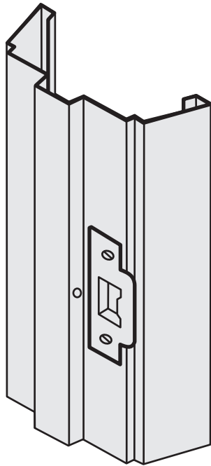
STANDARD STRIKE ASSEMBLY 1-1/8" X 2-3/4" (29 X 70)
